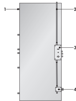
Fast-Sblock REI 30-60-90
