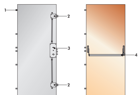
Sblock-Push REI 30-60-90
